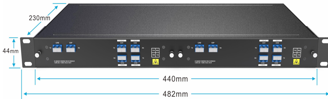
2-Slot 1U Rack for FMUC Module
