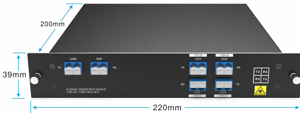
FMUC Plug in 2-Slot 1U Rack
