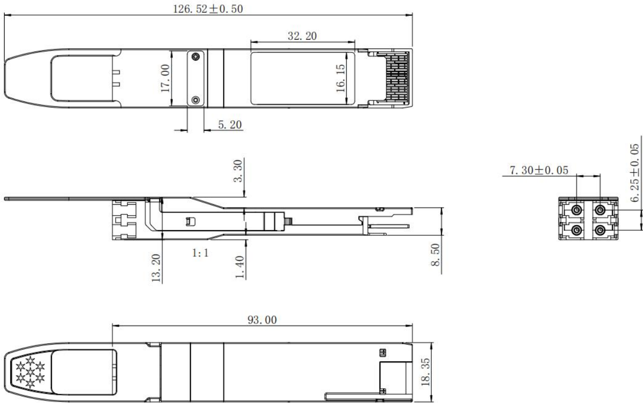
Figure6. Mechanical Specifications
