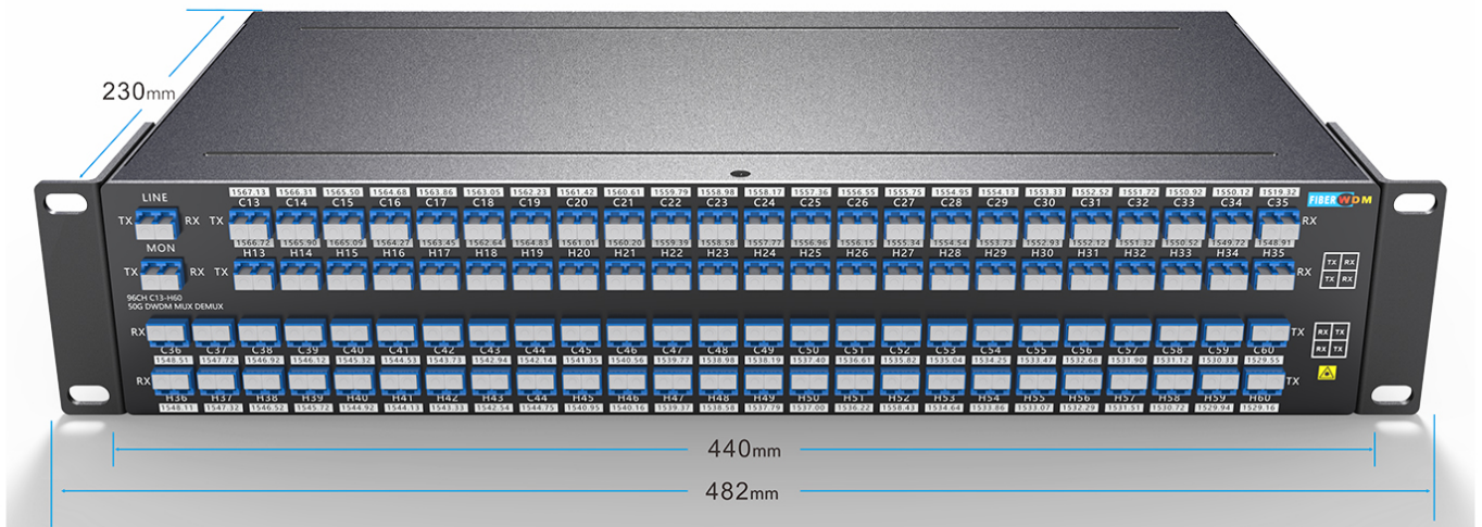
96CH DWDM 1U RACK
