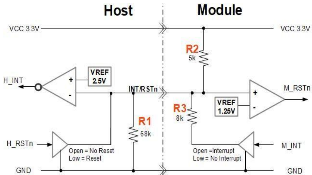
Figure 3 INT/RSTn circuit
