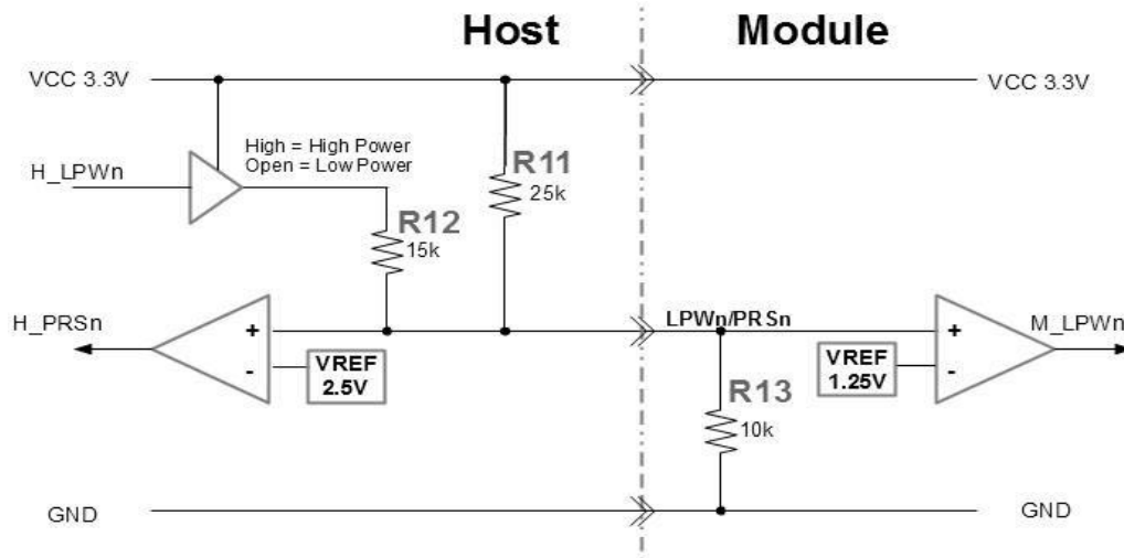
Figure 2 LPWn/PRSn circuit
