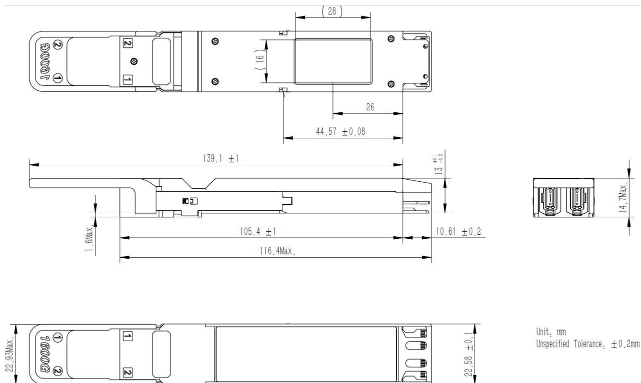
Figure 6 Package Outline
